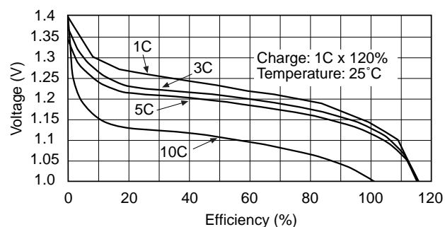
Discharge Curves of High Drain Series at Various Rates
